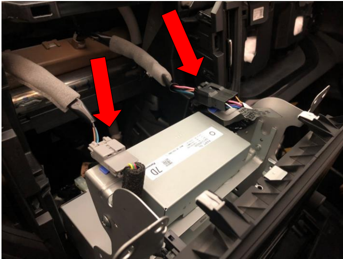
Disconnect two top connectors
