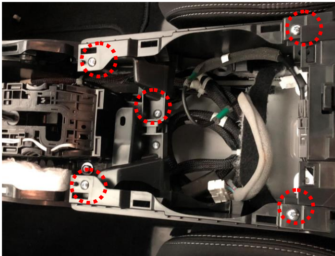
Remove five (5) Philips head screws
