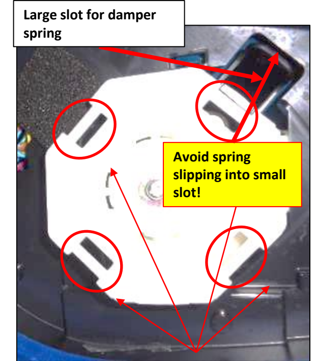
Backing Plate Housing clip holders
